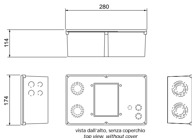
scatola terminali in alluminio per compressori V, Z W terminal box in aluminium for V, Z W compressors
